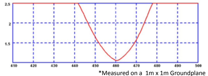
Typical VSWR*
