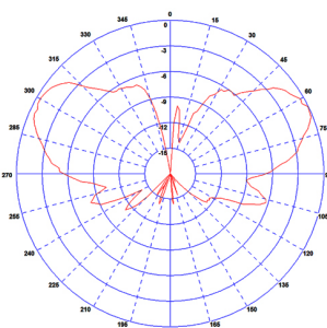
Typical E-Plane(2450MHz)
