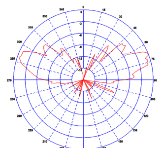
Typical E-Plane (5600MHz)
