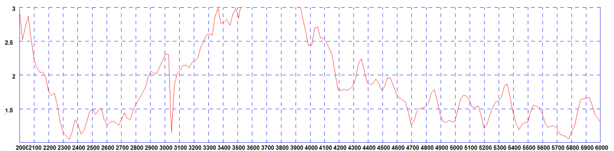
Typical VSWR*
